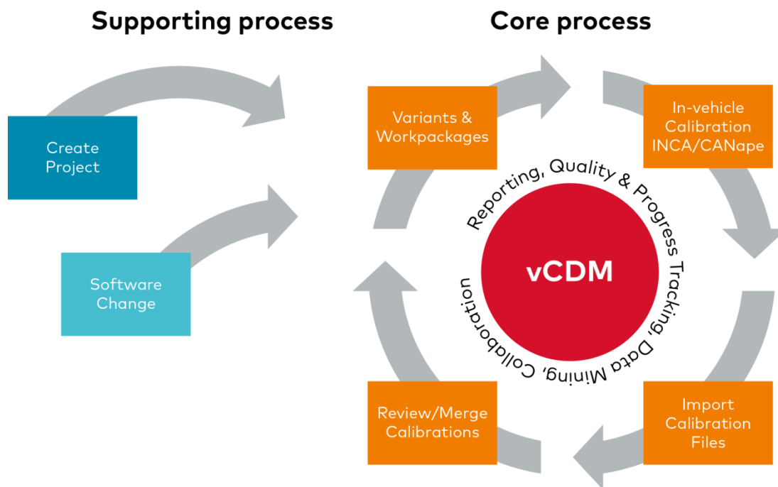
Figure 26: Overview calibration process in vCDM
