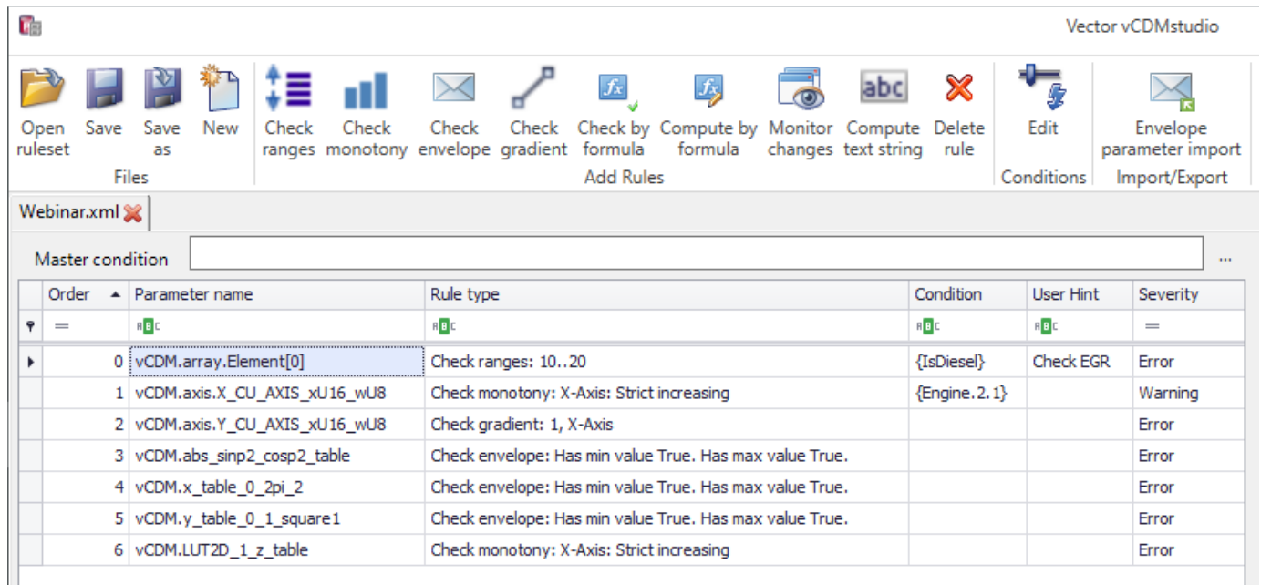
Figure 5: vCDM Ruleset Editor
