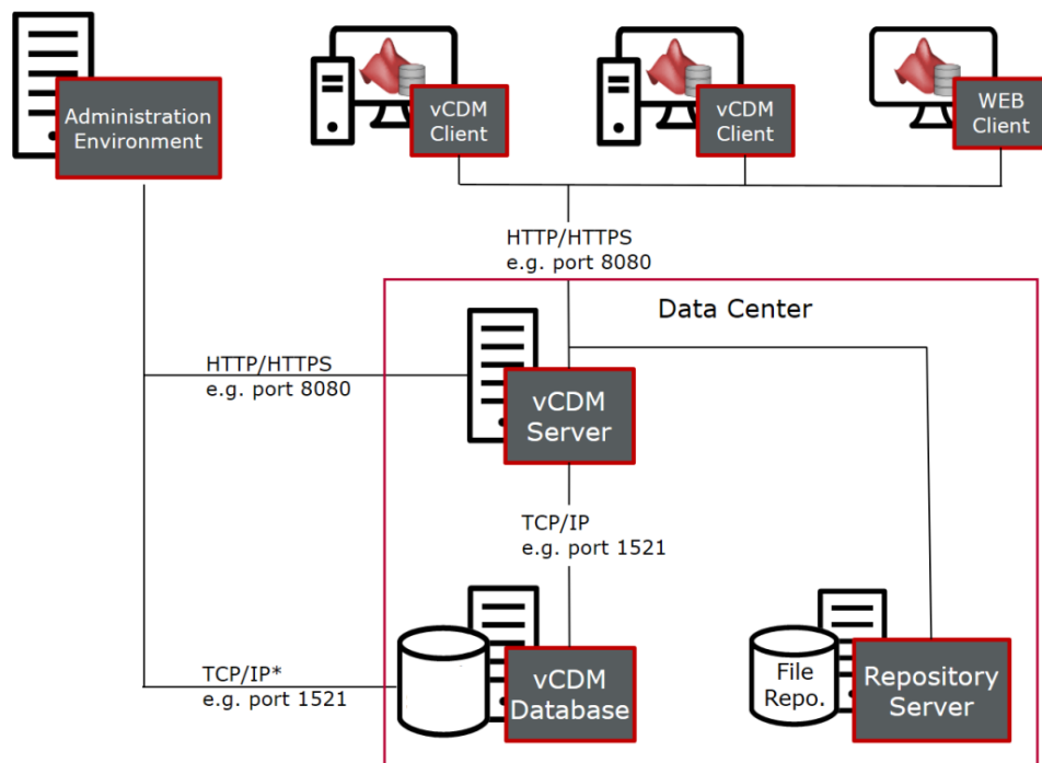
Figure 36: vCDM 3-Tier architecture
