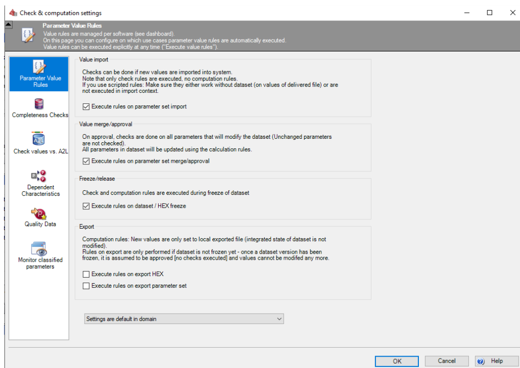
Figure 28: Setup Required Data Quality for the vCDM Validation Framework
